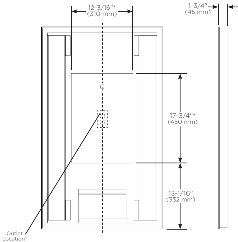
Back view for electrical outlet location
