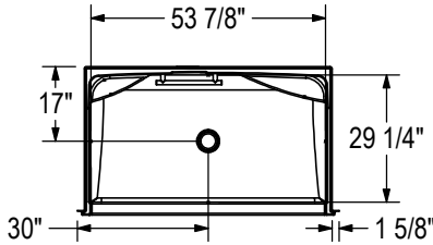
STANDARD (Left shown, Right symmetrical) 1-PIECE MODEL SHOWN
