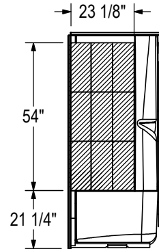
OPTIONAL REINFORCEMENT (Left shown, Right symmetrical)
