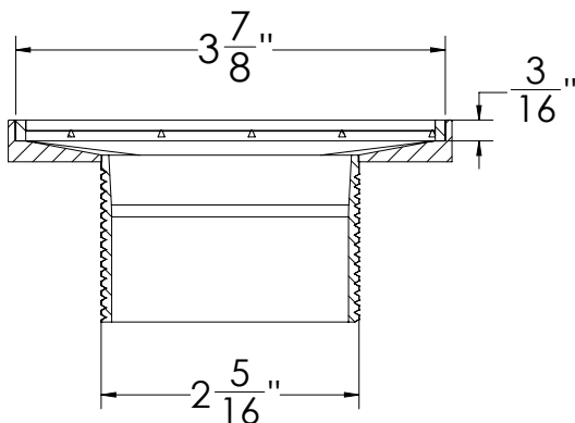
SECTION 1-1
