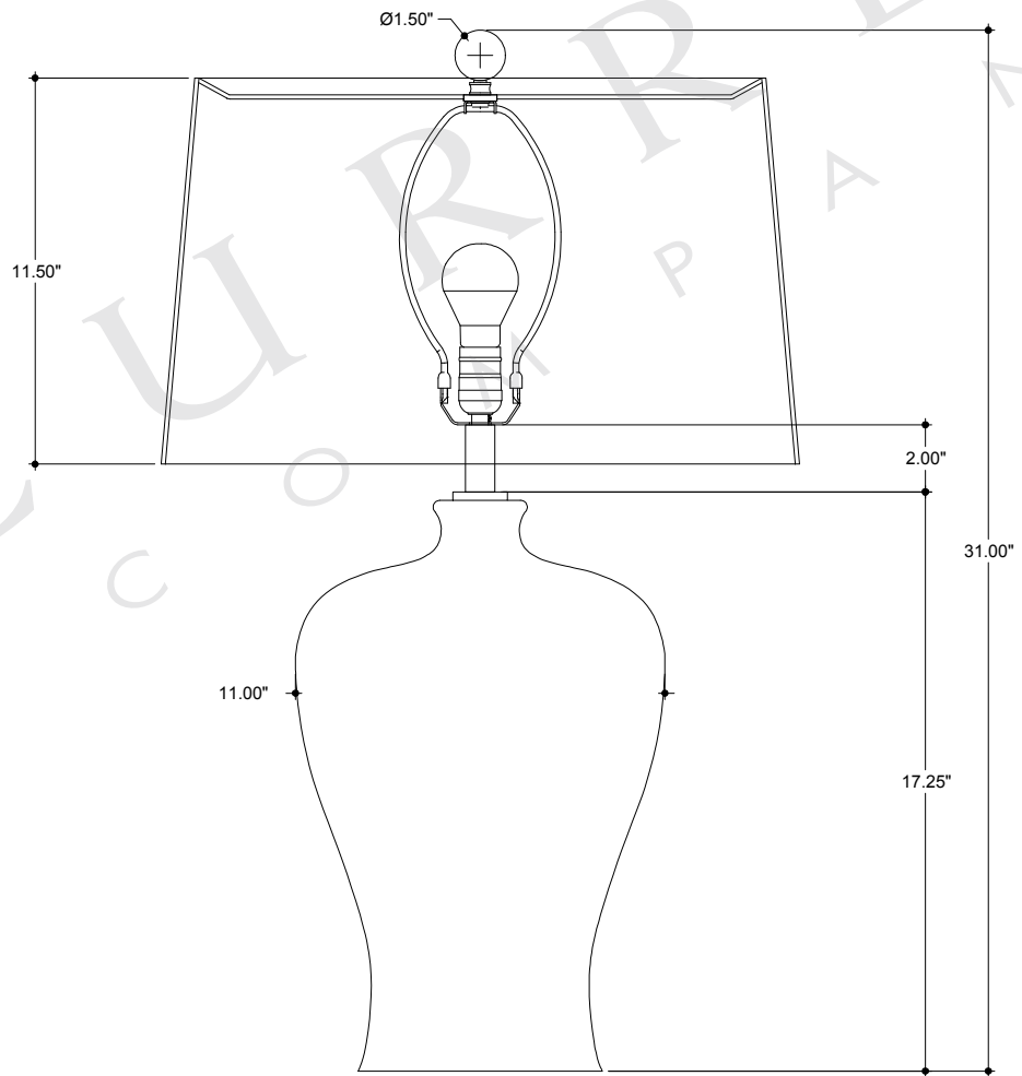
FRONT VIEW
