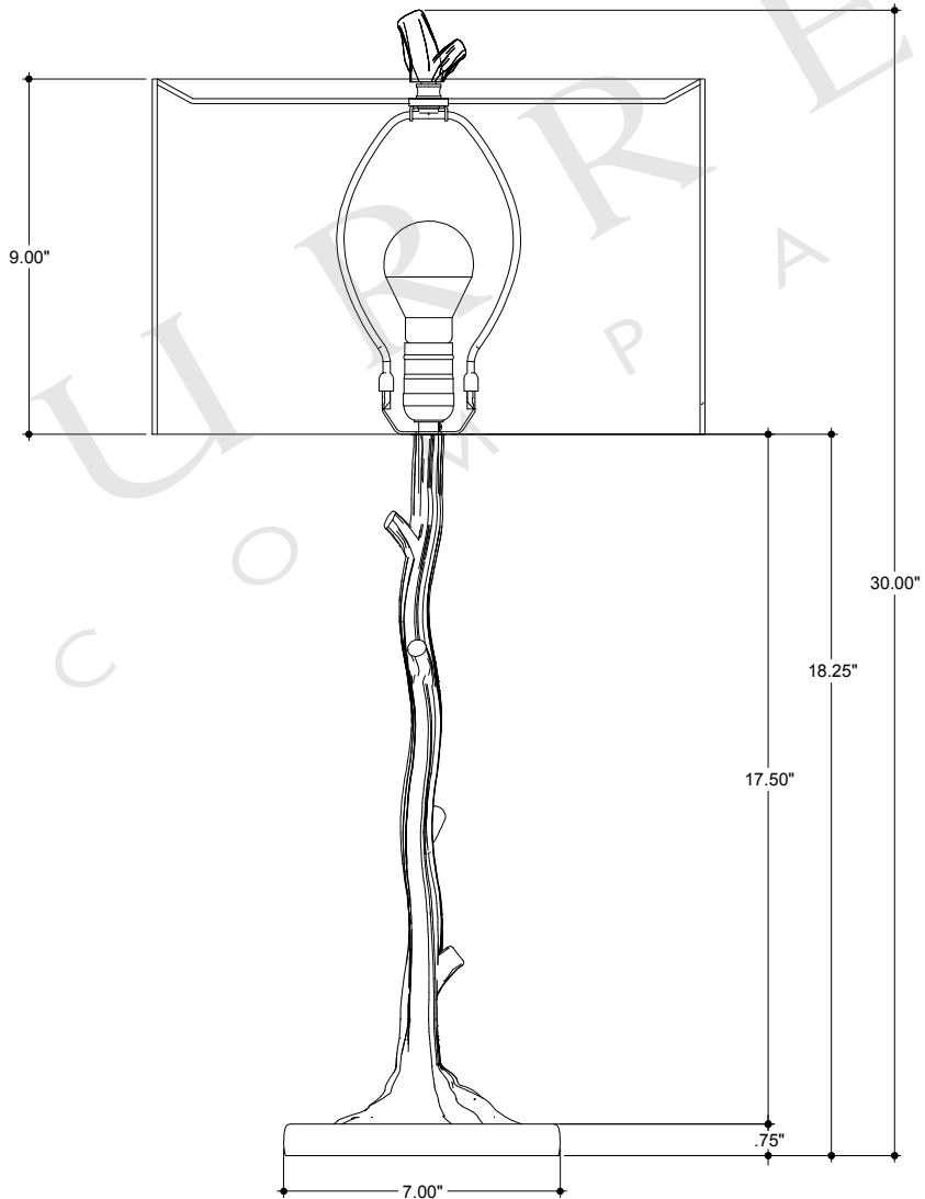
FRONT VIEW
