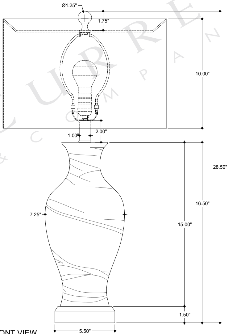
FRONT VIEW
