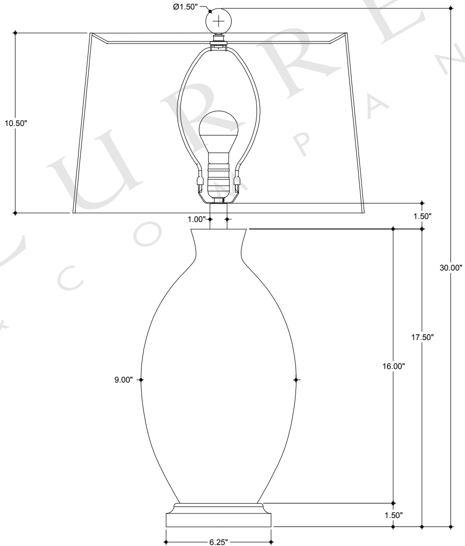
FRONT VIEW
