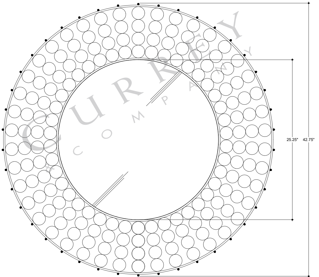
FRONT VIEW
